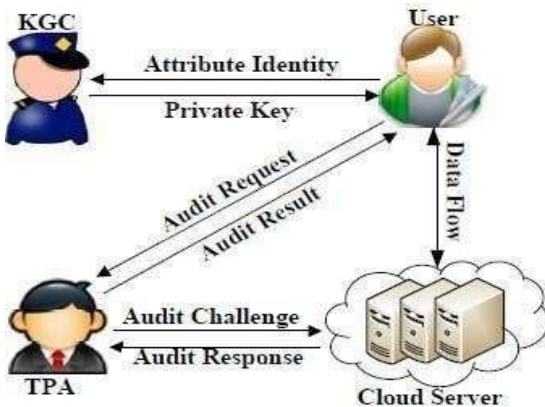
Fig. 1. The system model of attribute- based data integrity auditing protocol
