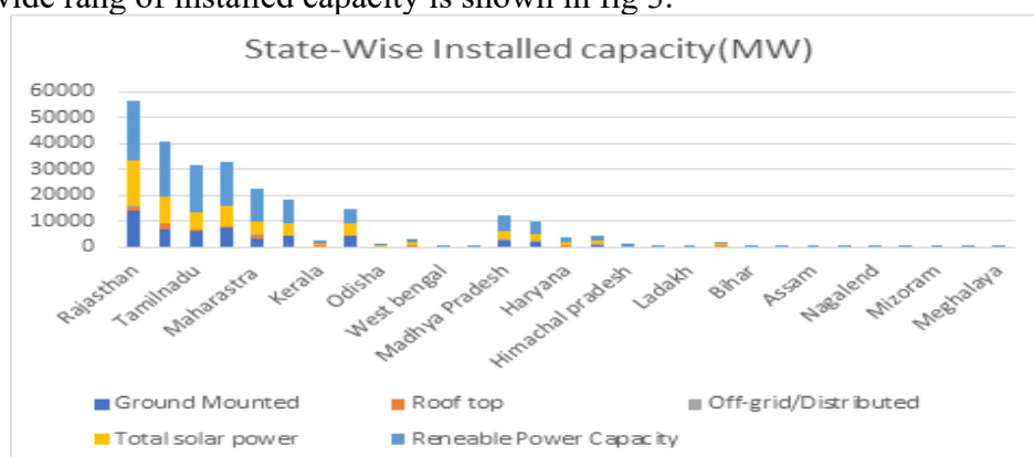
Fig 3: State-wise Installed capacity of Interactive renewable Power (MW)
