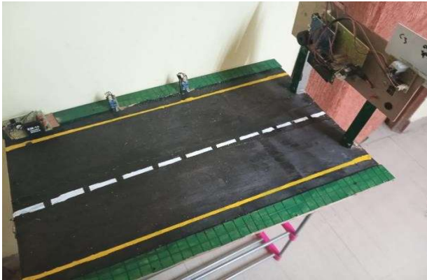
Fig. 3. Project Model
