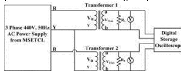
Fig. 3: Hardware Setup for Measuring phase angle & Magnitude between Line Voltages of two transformers
