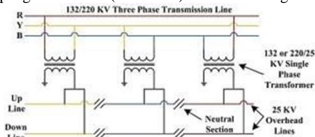
Fig.8: Schematic diagram of 25 kV overhead Traction lines
