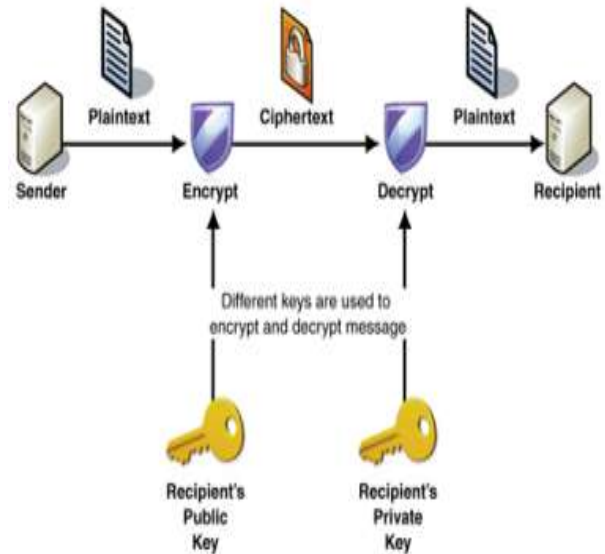
Fig. 2 Asymmetric Encryption Technique
