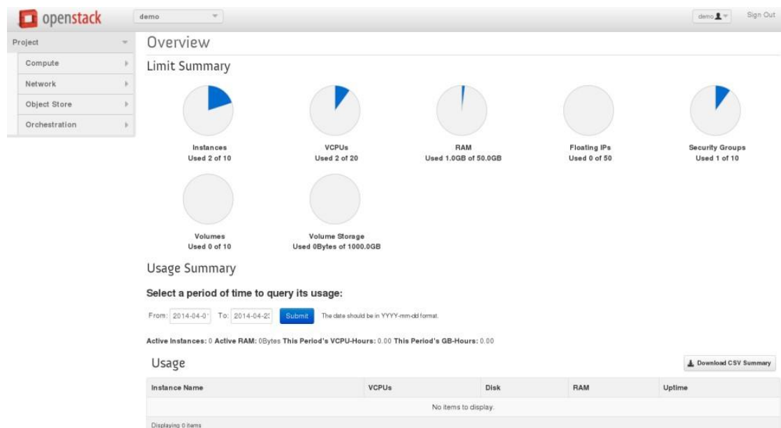
Figure 2: OpenStack dashboard [19].
