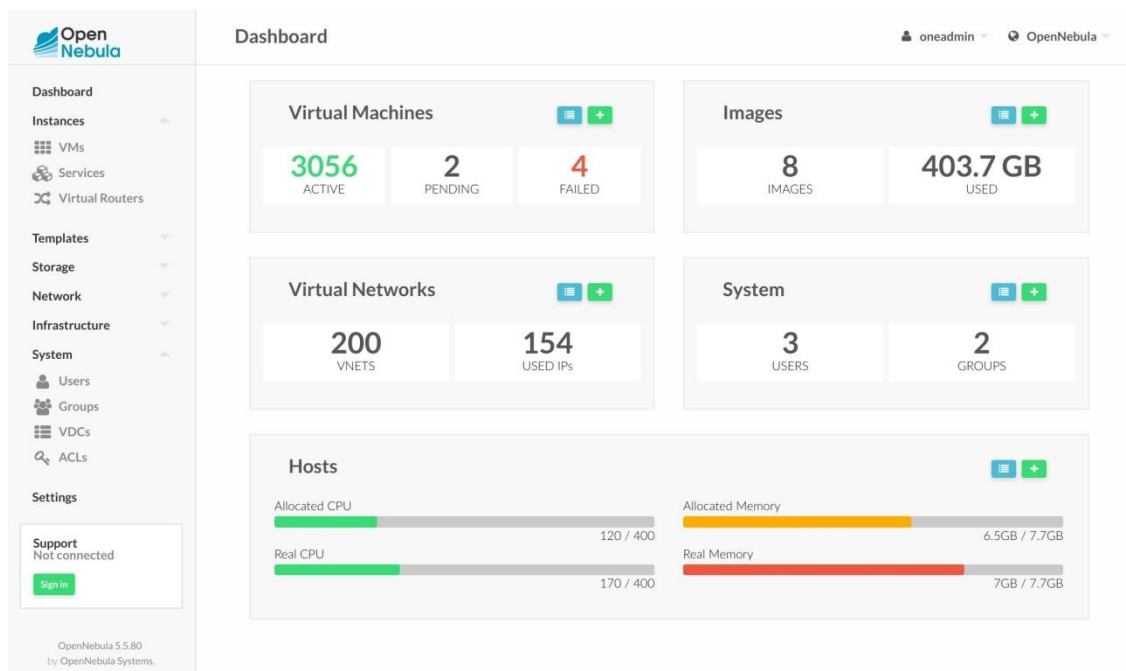
Figure 4: OpenNebula dashboard [27].
