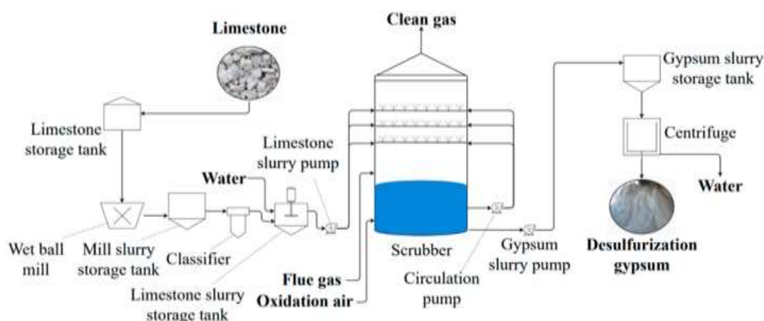
Figure 1:-Plant Layout for FGD Process for Gypsum
